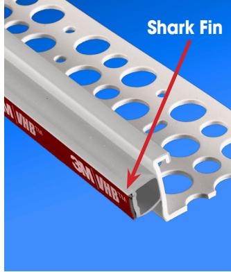
AMICO's Shark Fin Technology Ensures a Complete Waterproof Seal
